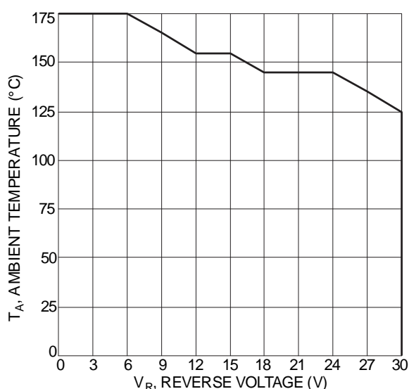
Figure 6 Reverse Voltage Derating
